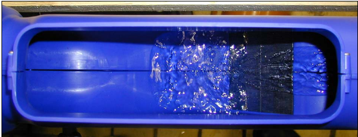
Figure 4: INTEWA Hydraulic jump filter WSP100 with Q = 0.1 \text{ l/s}
