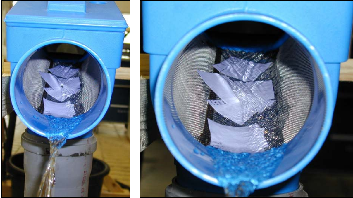
Figure 14: (left) 3P cartridge filter PF with Q = 0.2 \text{ l/s} and dirt (Paper)
