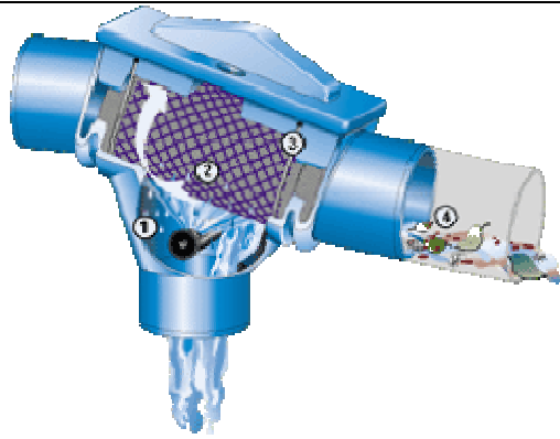
Figure 9: Functional principles of the backflushing automatic system of 3P cartridge filter PF
